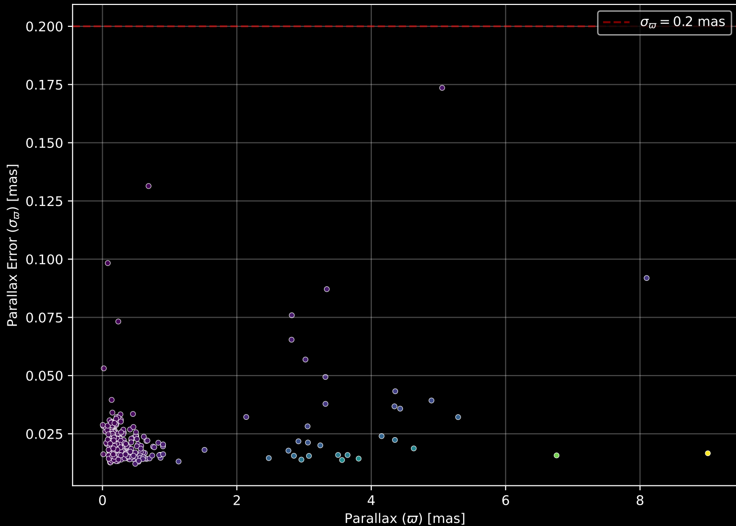
APOGEE DR17 Field: [214-08] Parallax Quality (n= 308)
