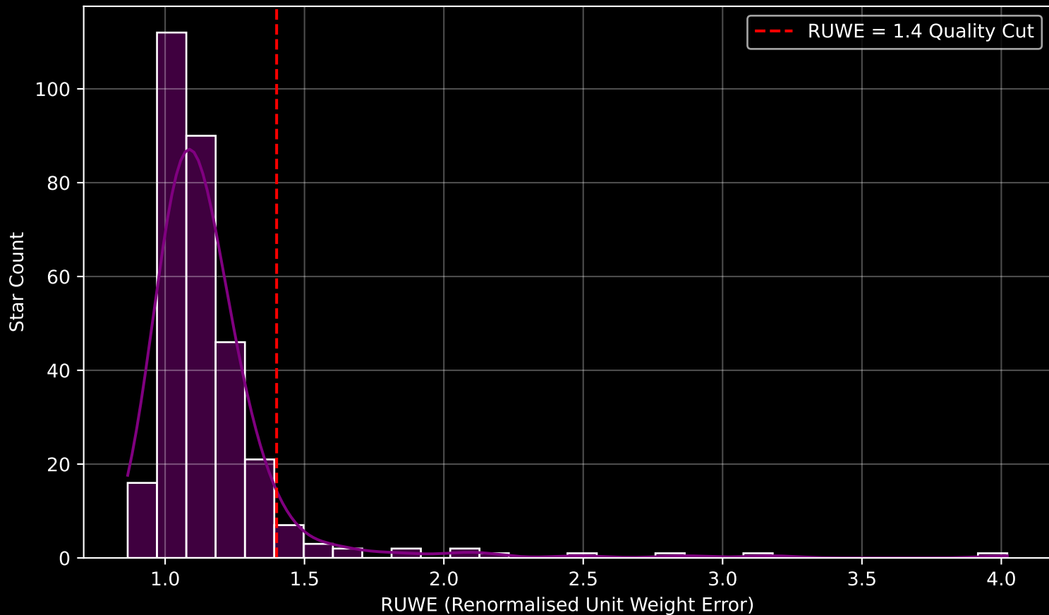
GAPOGEE DR17 Field [214-08] RUWE Distribution (n= 306)
