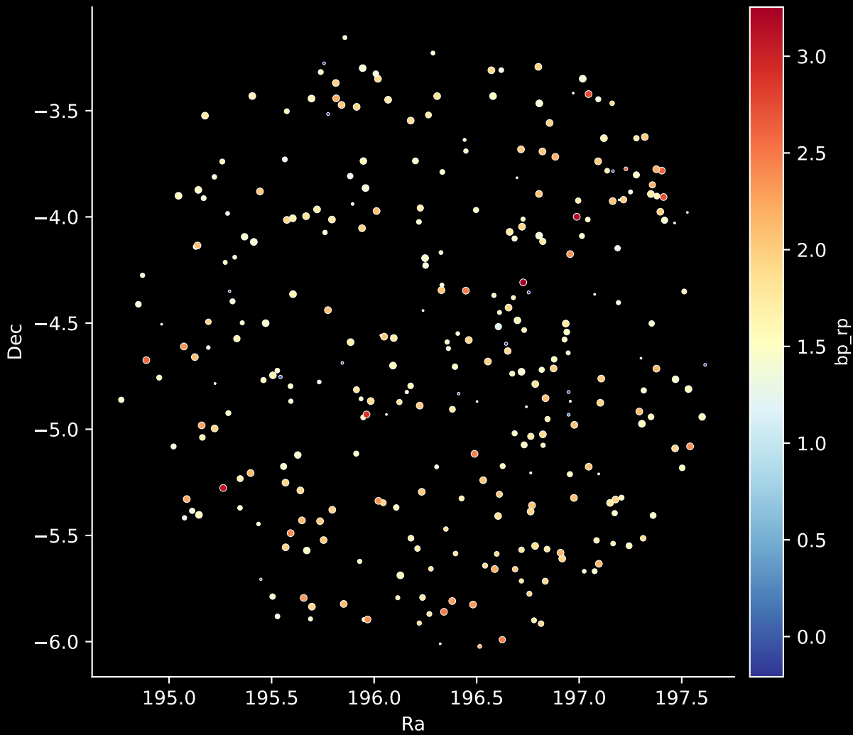
APOGEE DR17 Field: [214-08] Stars: 308
