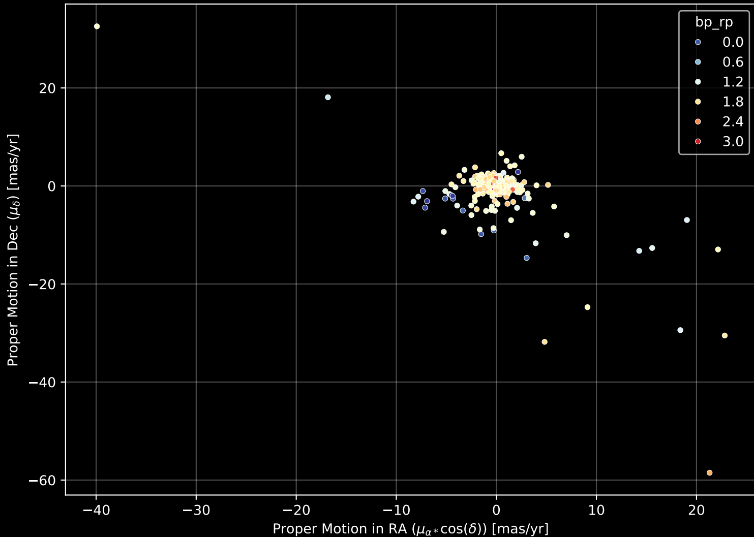
APOGEE DR17 Field: [214-08] Proper Motion Diagram (n= 308)
