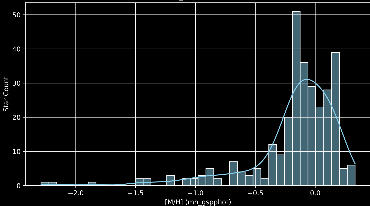
APOGEE DR17 Field: [214-08 [M/H] (mh_gspphot) (n= 303)
